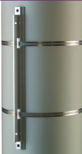
Bell Wing Bracket RPBCTBW12 - 12" (50/Box) (Requires single strap) RPBCTBW18 - 18" (50/Box) RPBCTBW24 - 24" (25/Box) Sign attaches with 5/16" bolts. Hardware NOT Included.
